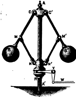
FIG. 29.—The Governor.
